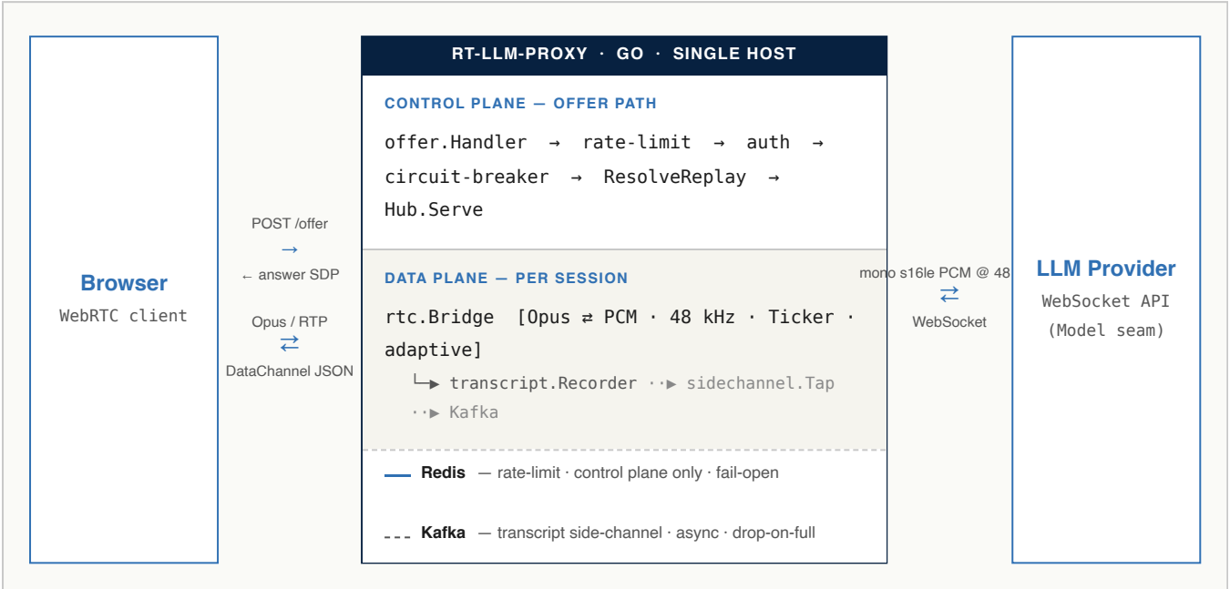
Figure 1. RT-LLM-Proxy system architecture. The control plane handles SDP offer negotiation, rate limiting (Redis, fail-open), authentication, per-provider circuit breaking, and session replay resolution — all on the offer path, never in the media loop. The data plane runs per session: rtc.Bridge terminates the WebRTC peer connection, transcodes Opus ↔ PCM, and paces outbound frames via a session-level Ticker ; transcript.Recorder assigns monotonic sequence numbers shared by the data channel and the side-channel; and sidechannel.Tap publishes events to Kafka asynchronously (dashed path, best-effort, drop-on-full). Solid arrows are on the hot path; dashed are optional.
