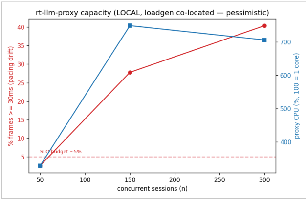
Figure 4. RT-LLM-Proxy capacity under co-located load testing (loadgen and proxy on the same 16-core host, loopback provider). Red: % frames \geq 30\text{ms} (pacing drift, SLO budget \sim 5\% dashed). Blue: proxy CPU (100 = 1 core). The SLO is healthy at n=50 (2.6%) and broken at n=150 (27.8%). These numbers are pessimistic — co-located loadgen steals \sim 3\text{--}7 cores from the proxy at n=50\text{--}150 .
