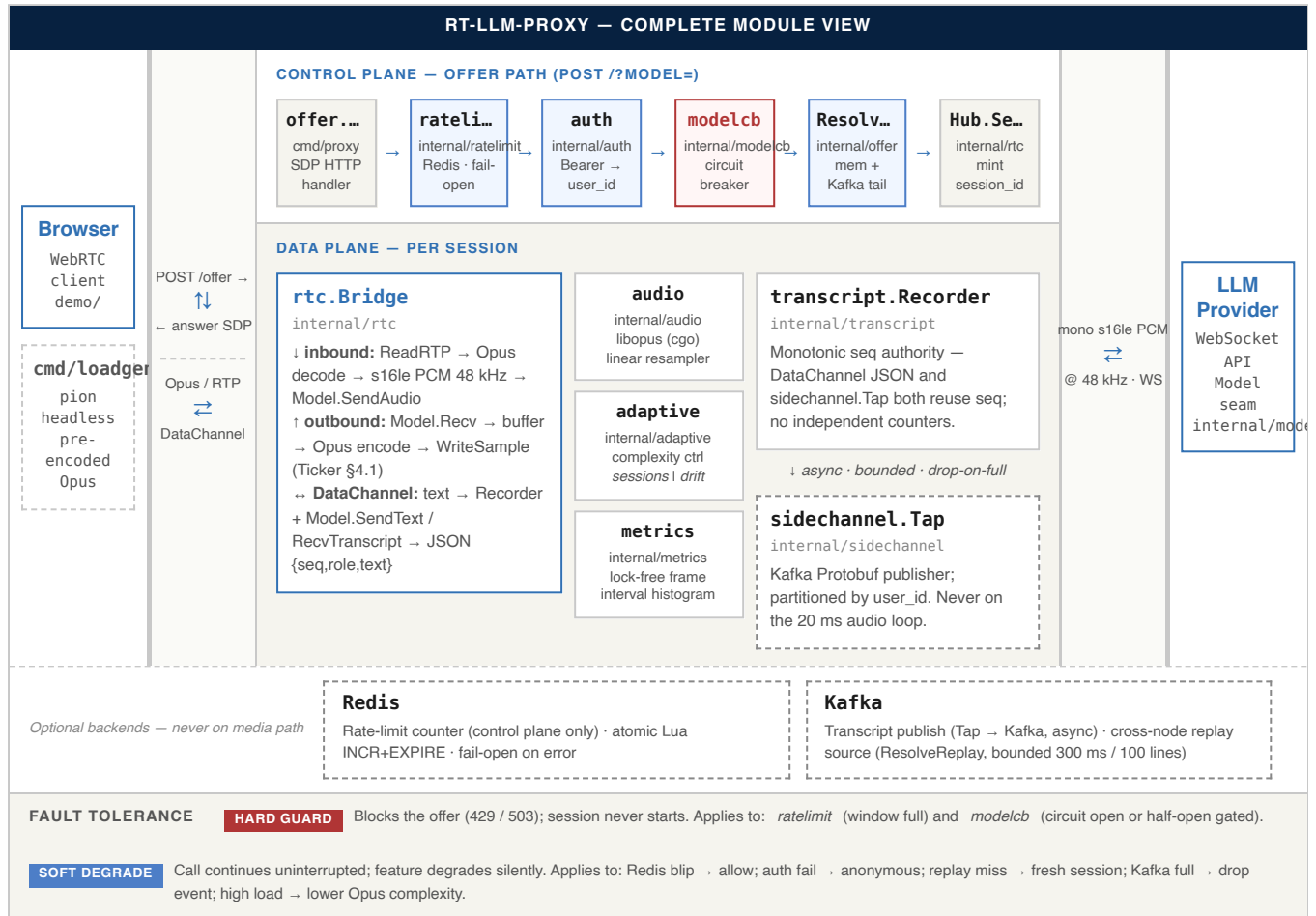
Figure 5. Complete module architecture. Solid borders = hot path; dashed borders = optional or best-effort paths. Blue-tinted boxes = soft-degrade on failure; red-tinted = hard guard. Arrows between the browser and the proxy, and between the proxy and the LLM provider, carry the audio and DataChannel traffic on the data plane, and SDP on the control plane.
